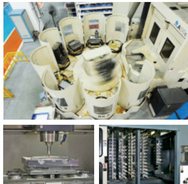
Standardized fixture can achieve single minute exchange of dies.
