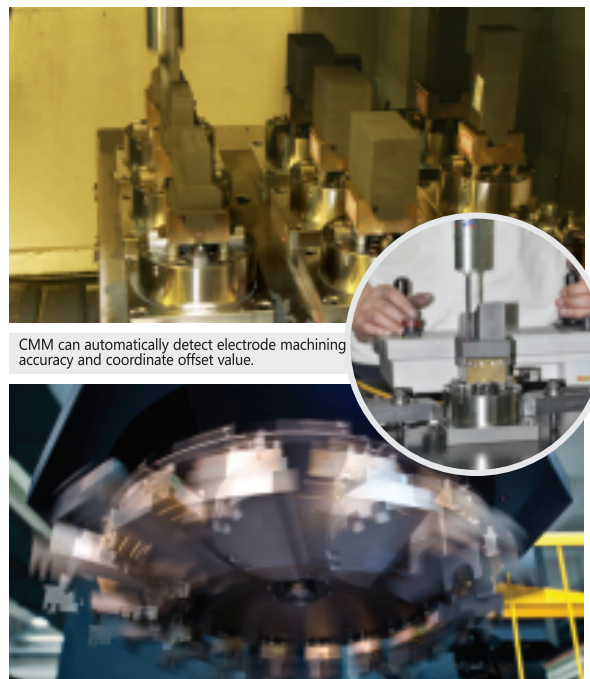
EDMCAM off-line programming and ATC applications achieves EDM automatic processing.
